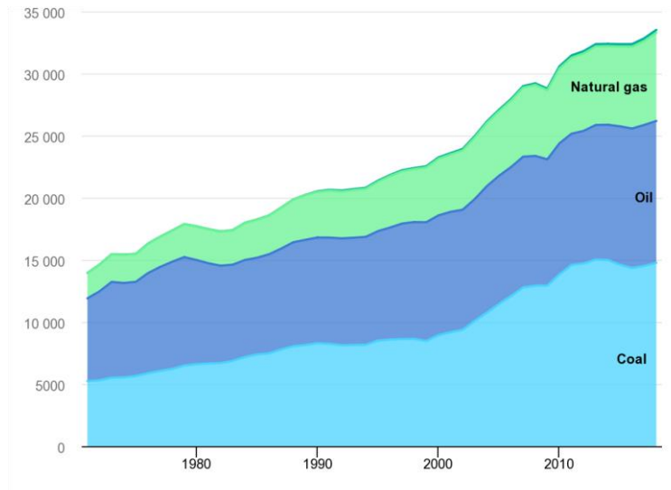
World CO2 emissions from fuel combustion, by fuel, 1971-2018, Mt 1
